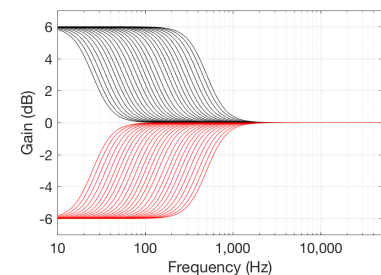
Figure 5.39: Magnitude Responses, low-shelving filter: F_c varied from 32 Hz to 500 Hz., Gain = \pm 6 dB, Q = 0.7 .
