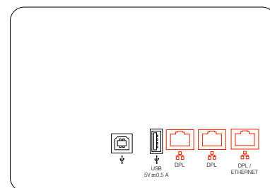
Figure 6.3: Audio connection panel – Secondary loudspeaker. The only audio connectors on this loudspeaker are for the Digital Power Link connection to the Primary loudspeaker.
