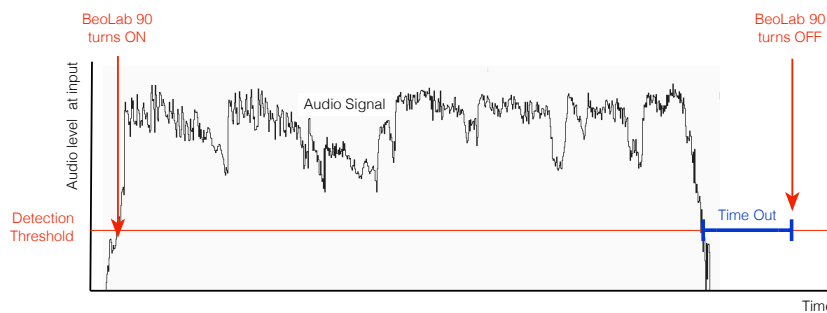
Figure 5.50: The "Detection Threshold" and "Time Out" parameters
