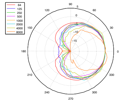
Figure 5.11: Polar plot of the directivity of the Wide Beam. Latency: Long
